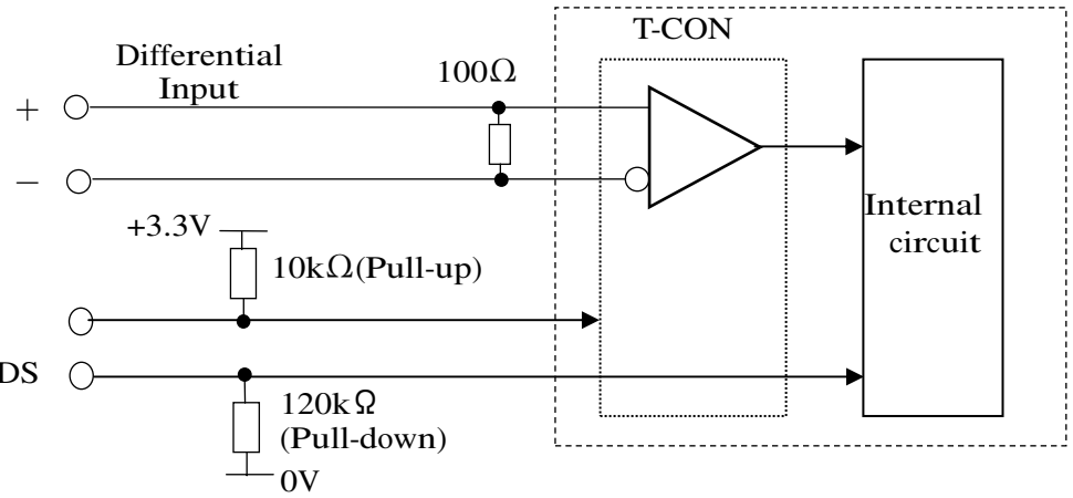
Figure 8-2(A) Equivalent circuit of logic signal Input
